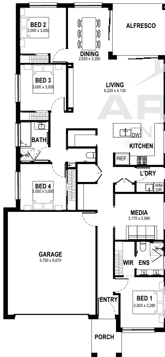
FLOOR PLAN
