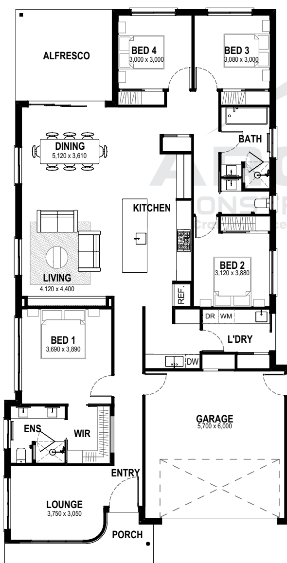
FLOOR PLAN
