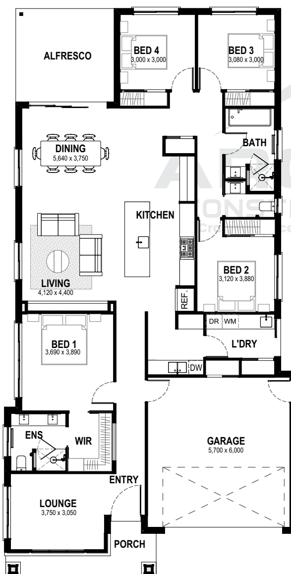
FLOOR PLAN
