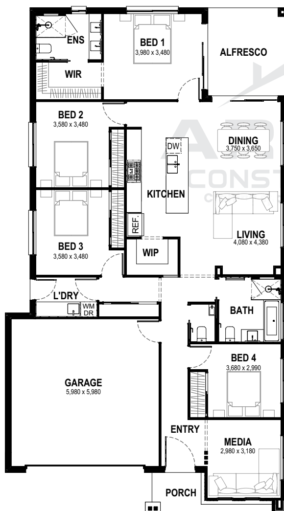
FLOOR PLAN
