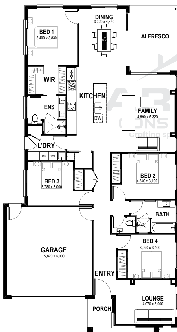
FLOOR PLAN
